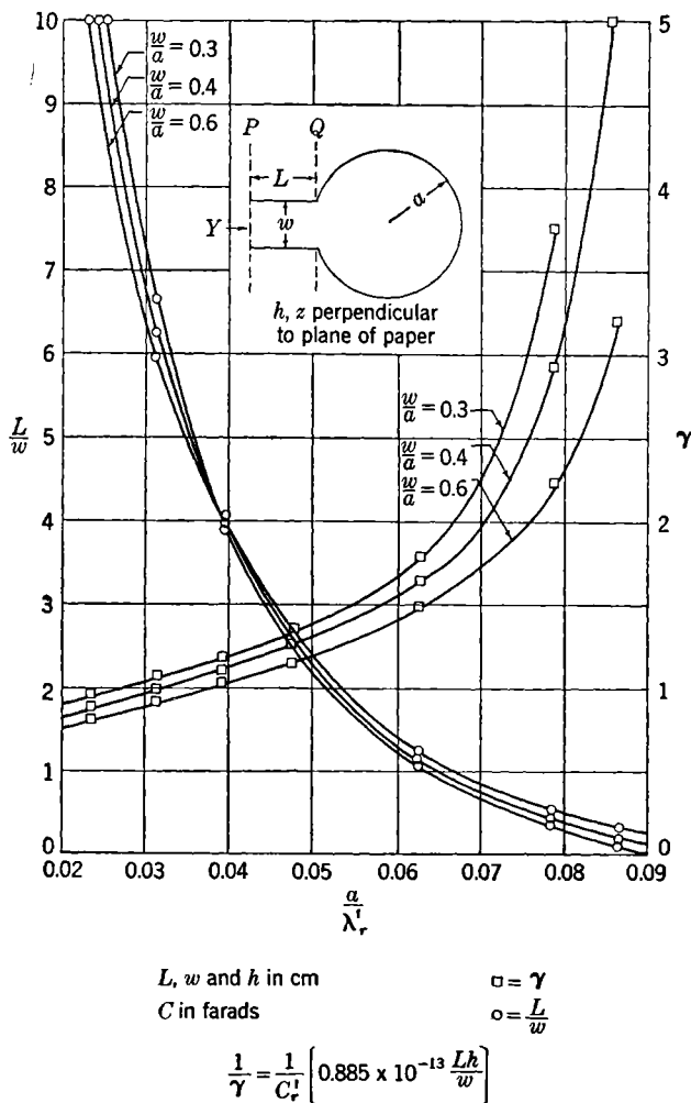
FIG. 11-4.—Circuit parameters of a hole-and-slot resonator.
